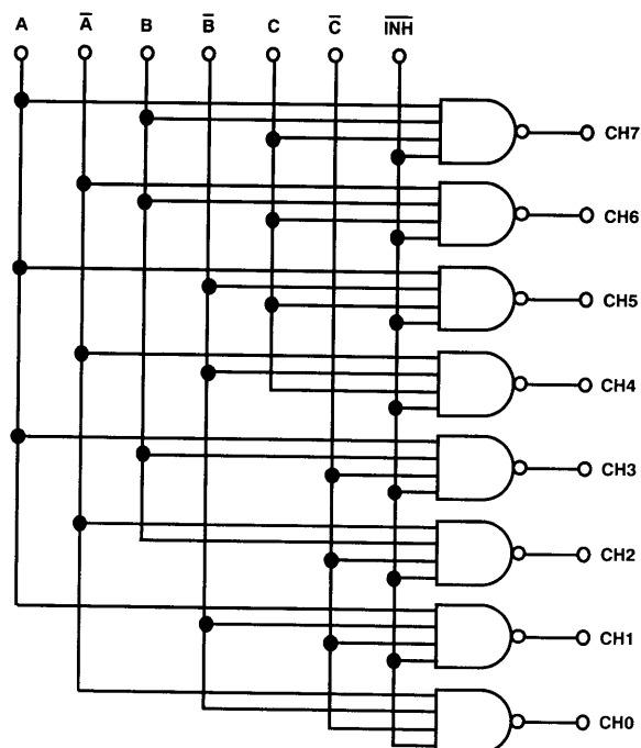
Figure 17. SMP-08/SMP-18 Decode Logic Diagram
