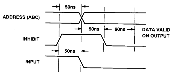
Figure 16b. SMP-08/SMP-18 Decode Timing Option 2
