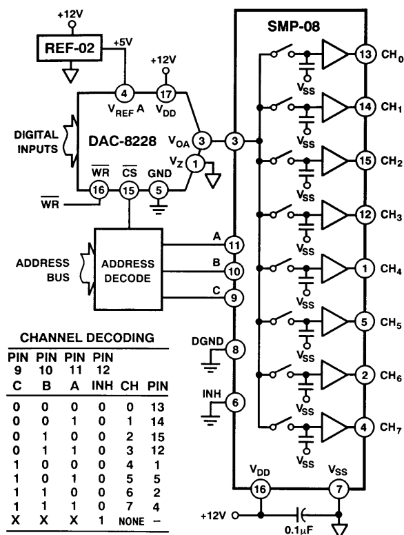
Figure 2. An 8-Channel Setpoint Controller
