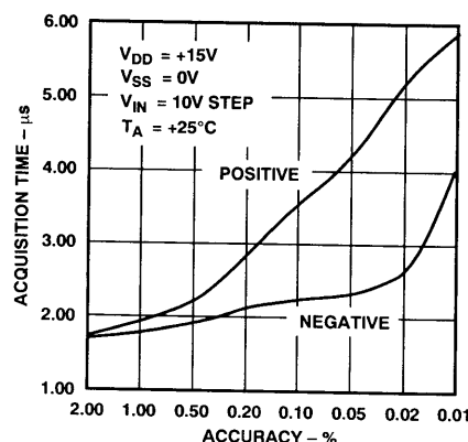
Figure 12a. SMP-04/SMP-08 Acquisition Time vs. Percent Accuracy
