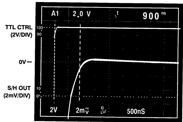
Figure 15c. SMP-04/SMP-08 Output Buffer Response to a 1 mA Load Current Transient. V_{DD} = +5\text{ V} , V_{SS} = -5\text{ V}
